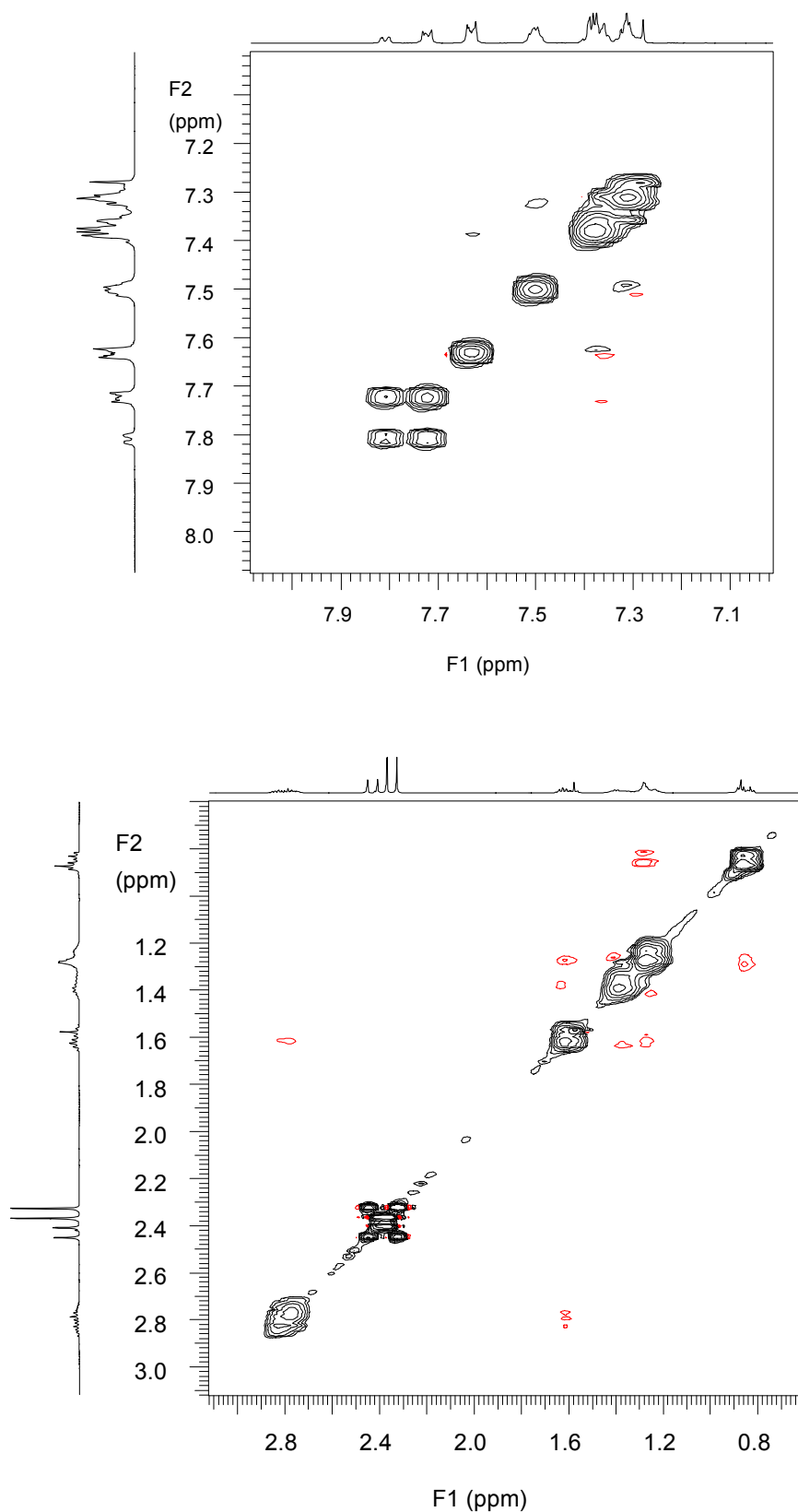
Figure S1: The aromatic (top) and aliphatic (bottom) part of the NOE experiment carried out on 23. Red peaks mark the NOE effect and the black peaks show the exchange between the two conformers, which is especially clear for the multiplets at 7.80 and 7.72 ppm, respectively (top) and the SMe singlets at 2.43-2.31 ppm (bottom).
